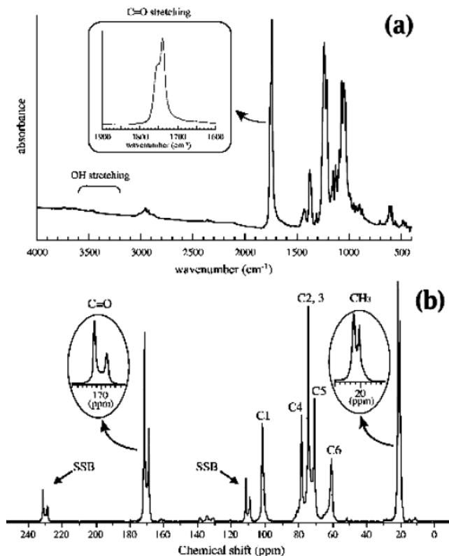
Figure 2. (a) FT-IR spectrum of CTA I. The bands of the indicated OH stretching region, characteristic of cellulose, do not appear on the spectrum. (b) Solid-state ^{13}\text{C} NMR spectrum of CTA I. See text for description. SSB indicates spinning sideband.
